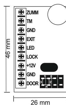
Figure 2: Controller PCB layout
