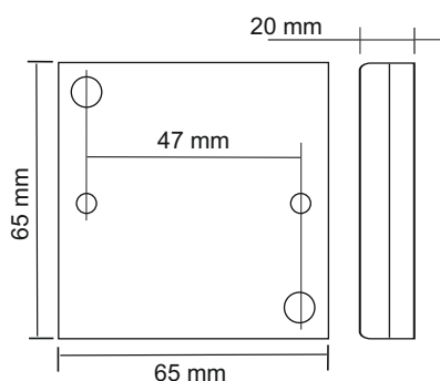
Figure 1: Controller case dimensions
